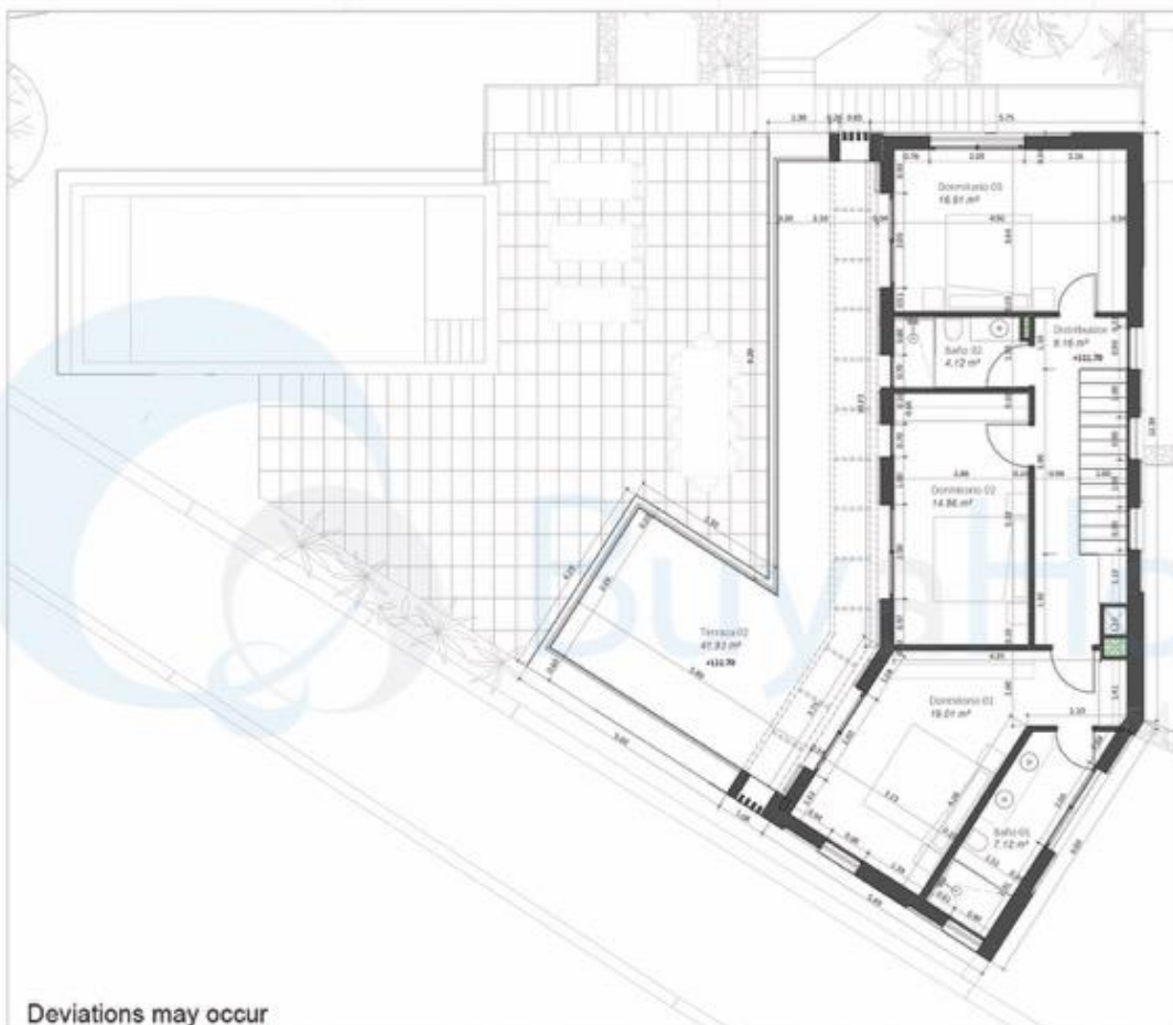
PLANO Ground Floor. Layout, surfaces and dimensions FORMATO: ESCALA: A3 1:75
