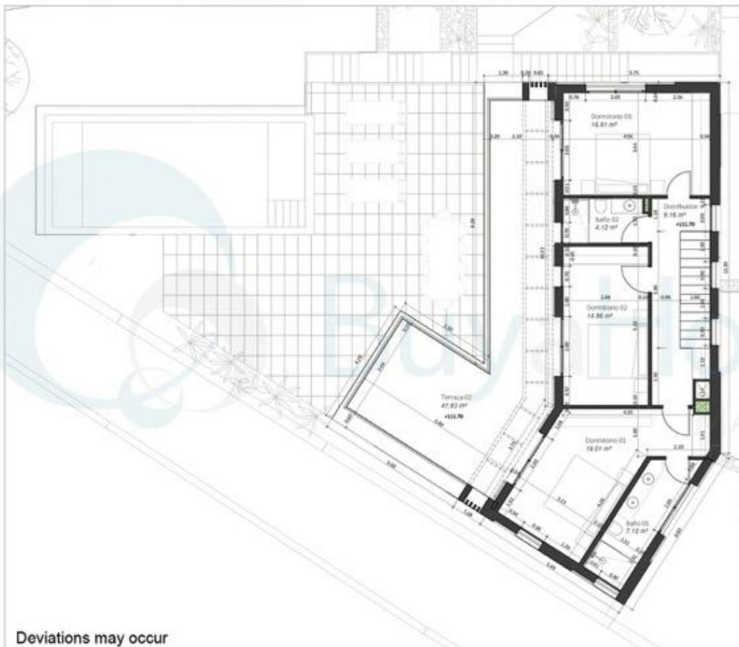
PLANO First Floor. Layout, surfaces and dimensions FORMATO: ESCALA: A3 1:75
