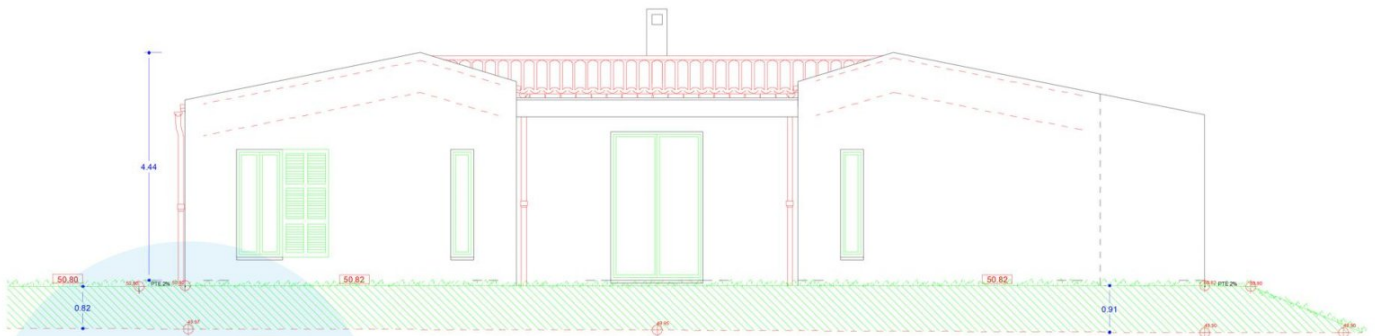
North elevation
